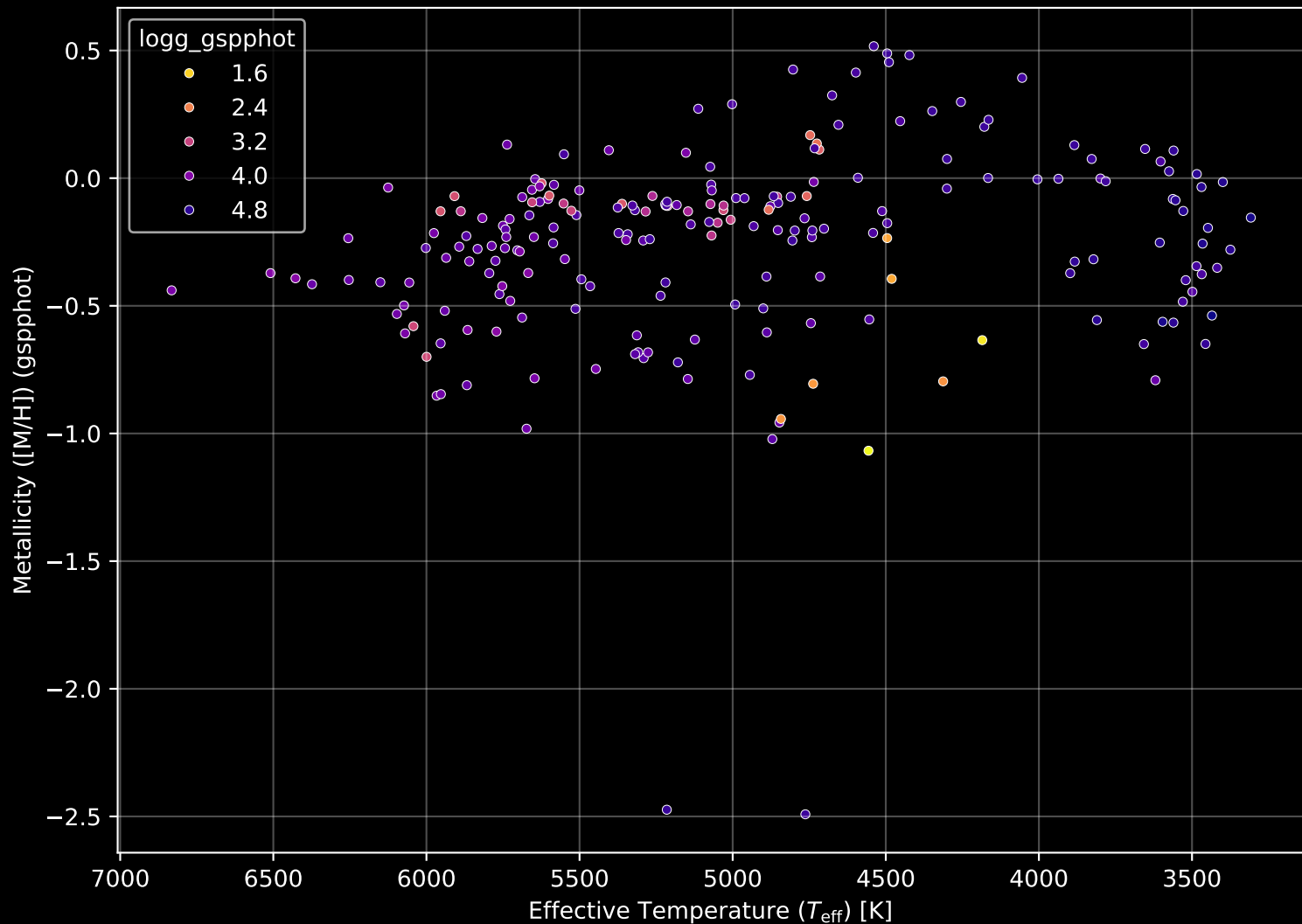
APOGEE DR17 Field: [K2_C8_133-52] Stellar Population Parameters (n= 216)
