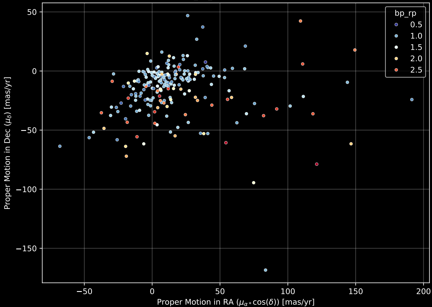
APOGEE DR17 Field: [K2_C8_133-52] Proper Motion Diagram (n= 216)
