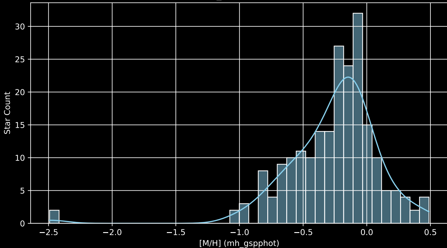
APOGEE DR17 Field: [K2_C8_133-52 [M/H] (mh_gspphot) (n= 215)
