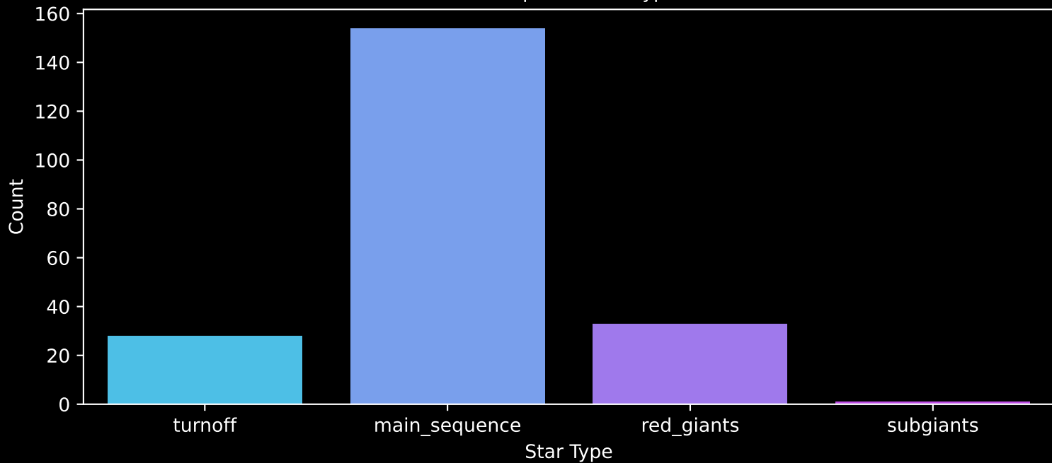
APOGEE DR17 Field: [K2_C8_133-52] Count plot of Star Type
