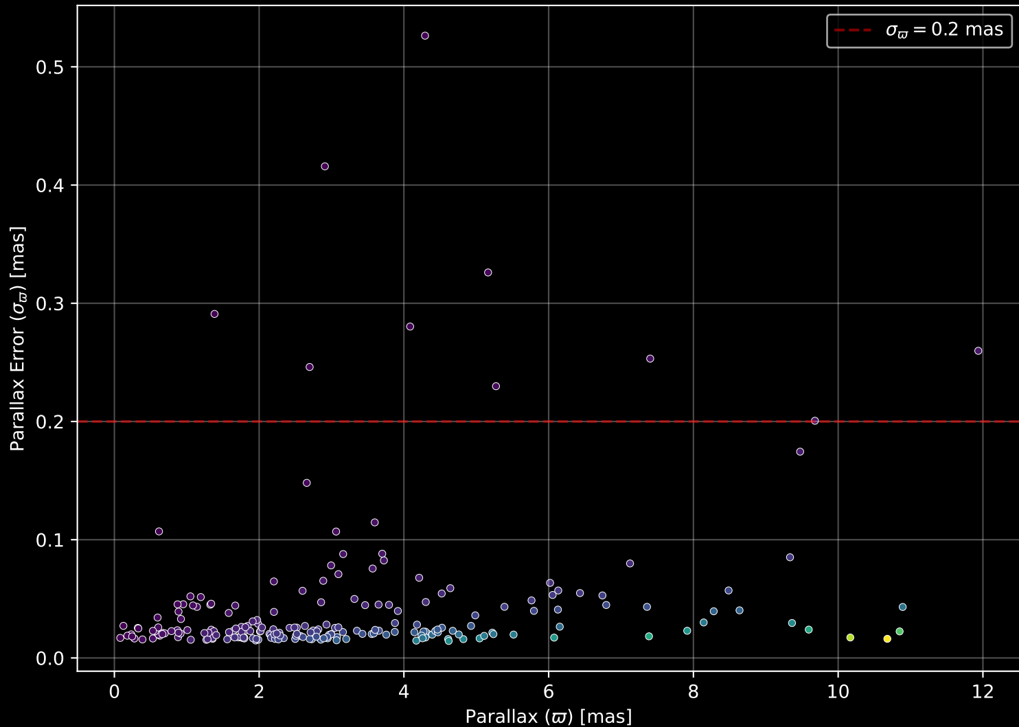
APOGEE DR17 Field: [K2_C8_133-52] Parallax Quality (n= 216)
