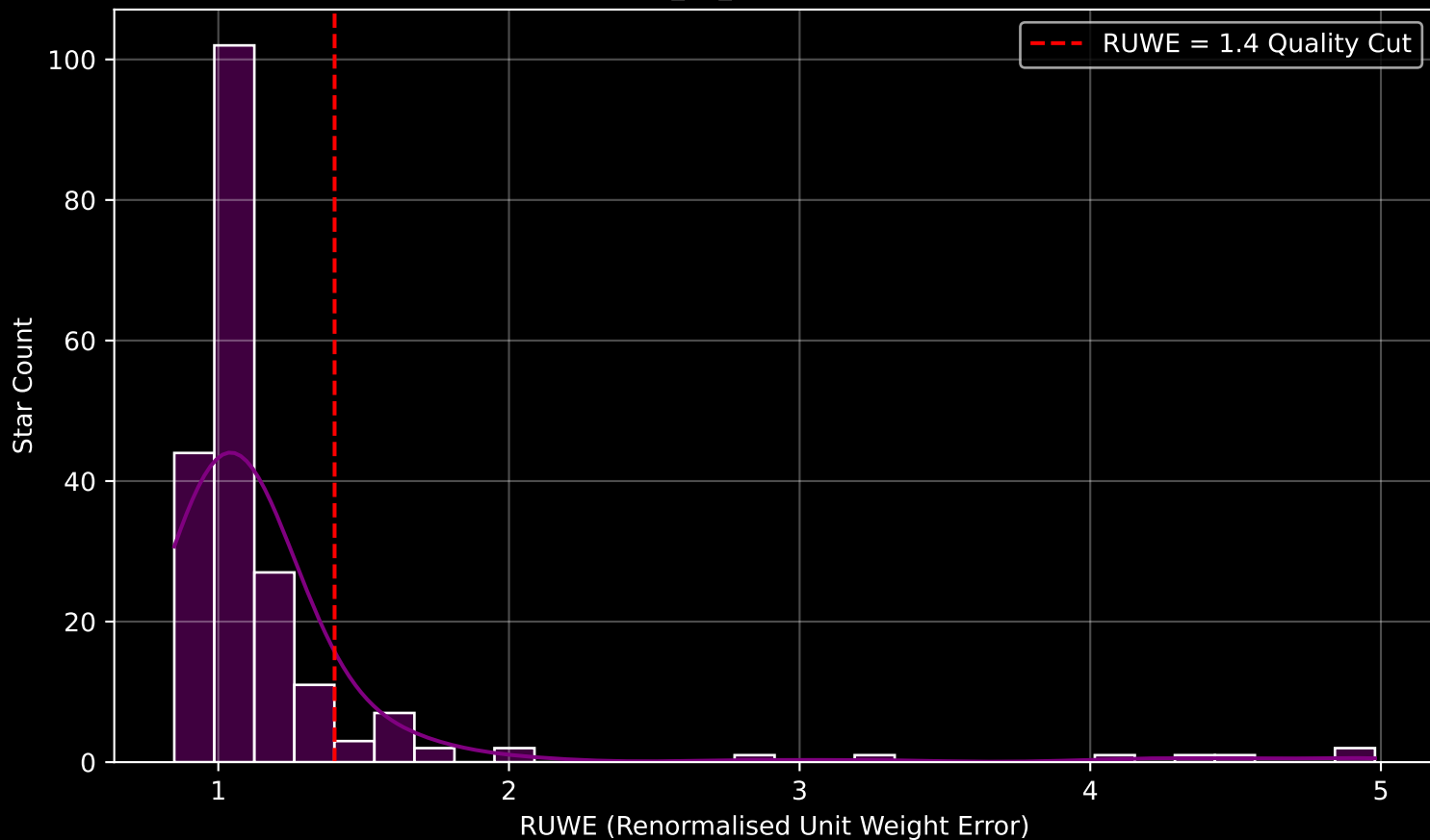
GAPOGEE DR17 Field [K2_C8_133-52] RUWE Distribution (n= 205)
