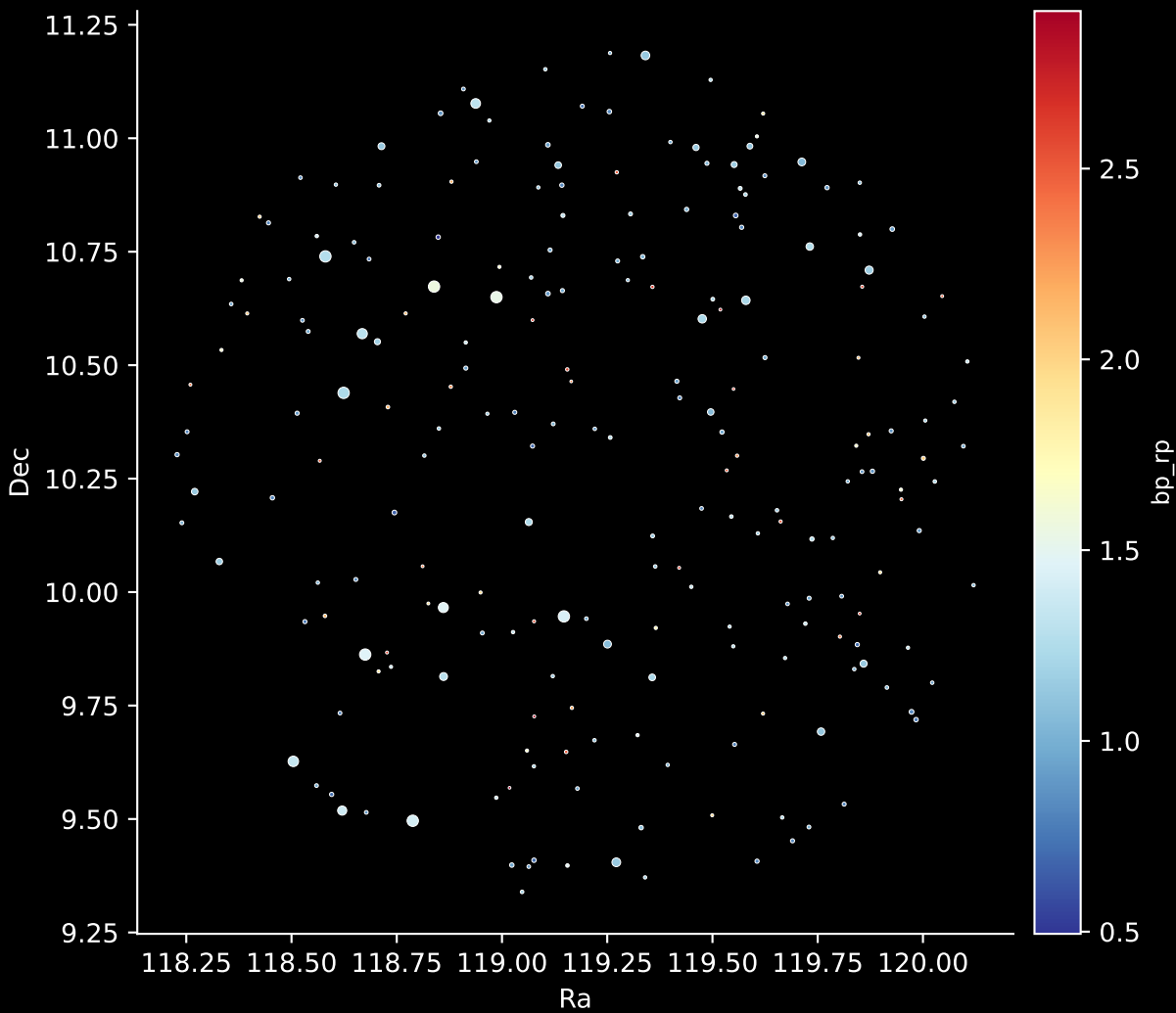
APOGEE DR17 Field: [K2_C8_133-52] Stars: 216
